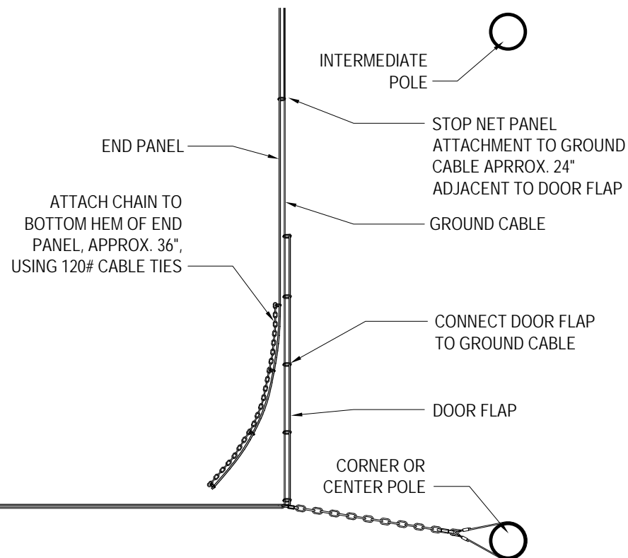
5 DOOR FLAP ATTACHMENT Scale: Not to Scale
