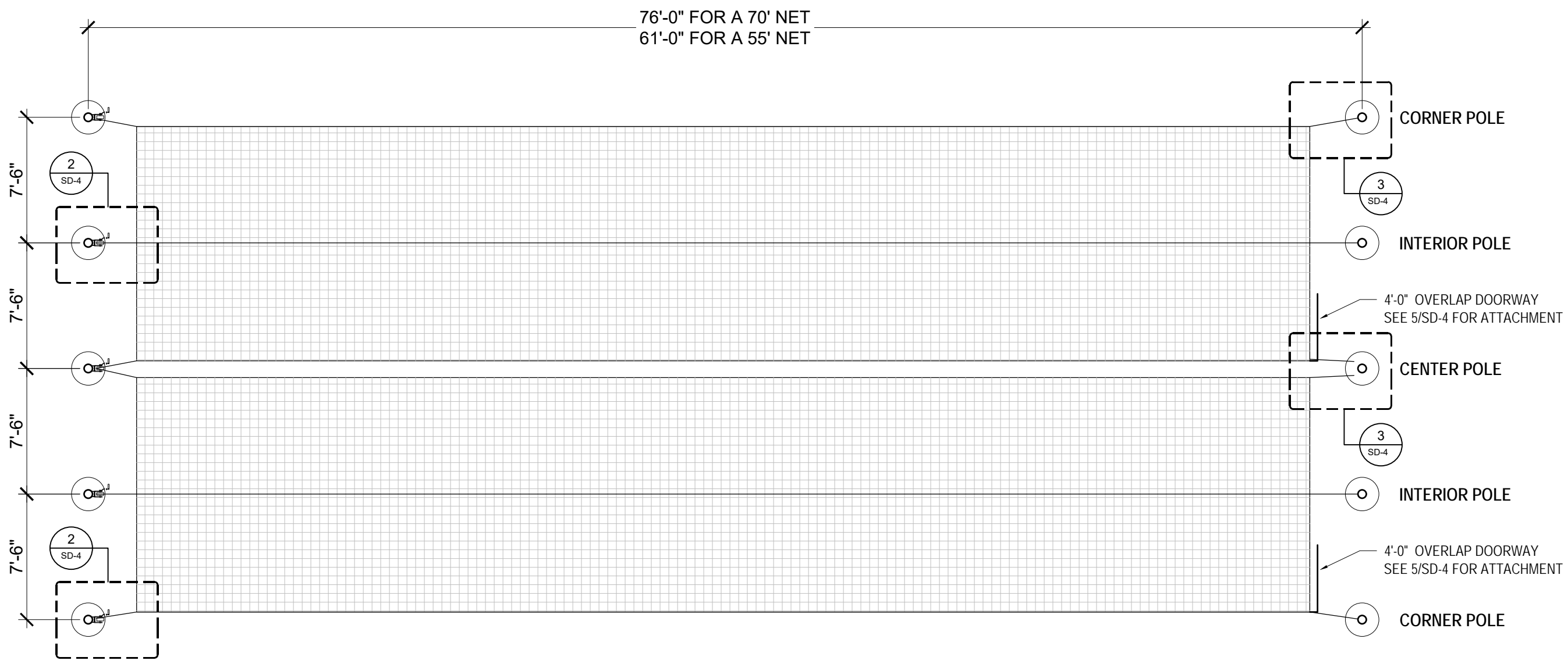
1 PLAN VIEW Scale: NOT TO SCALE
