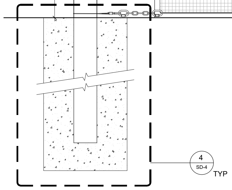
1 SIDE ELEVATION WHEN TENSIONED Scale: 3/4" = 1'-0"
