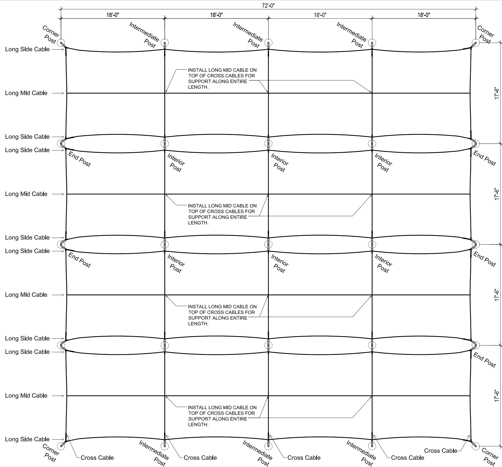
1 FOOTPRINT & CABLE LAYOUT Scale: 1/8" = 1'-0"
