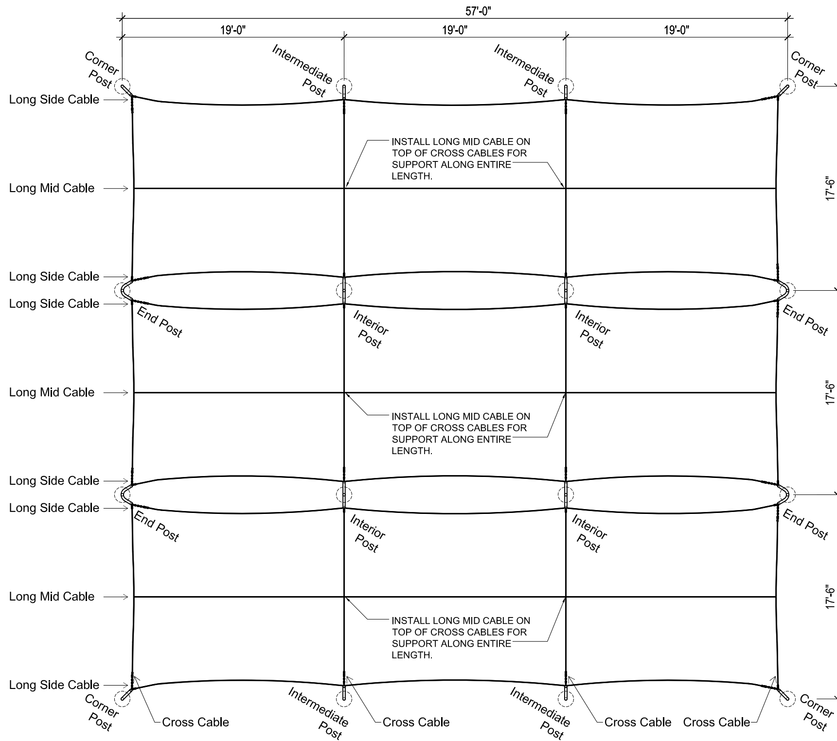
1 FOOTPRINT & CABLE LAYOUT Scale: 1/8" = 1'-0"
