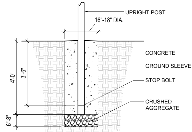
OPTIONAL GROUND SLEEVE
