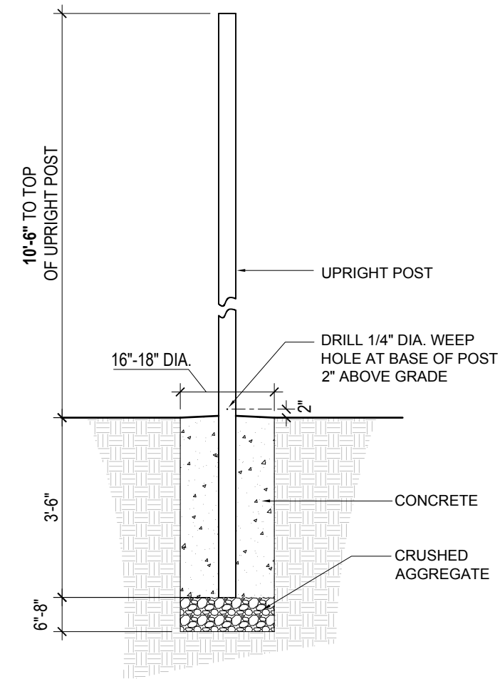
STANDARD DIRECT-BURY INSTALLATION
