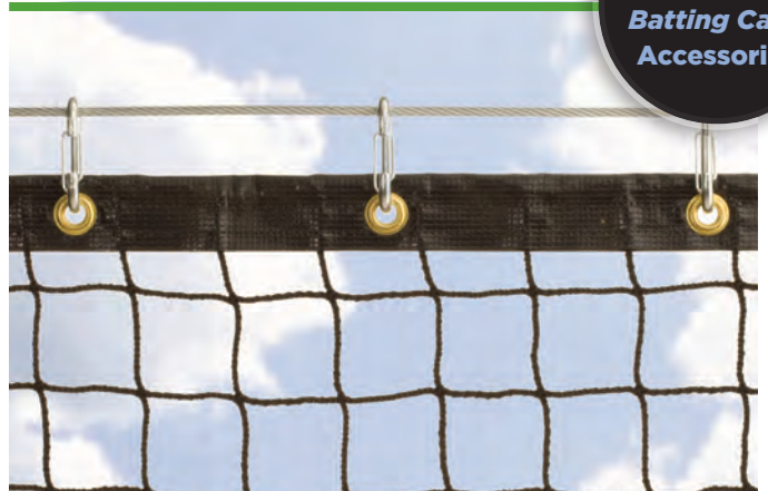
Steel clips and brass grommets for all net-to-cable connections.
