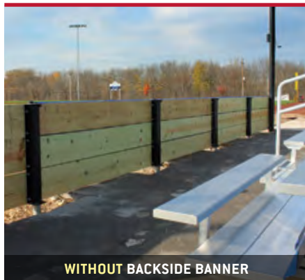
Slide-over Post Bracket with Net Anchor Cable
