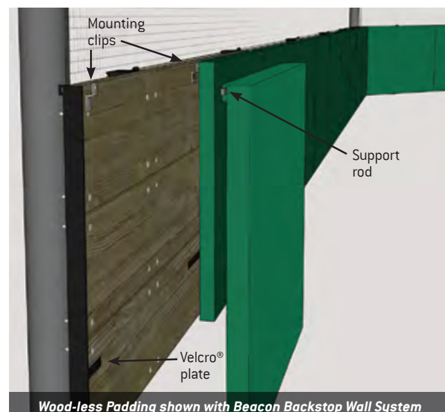
Wood-less Padding shown with Beacon Backstop Wall System
