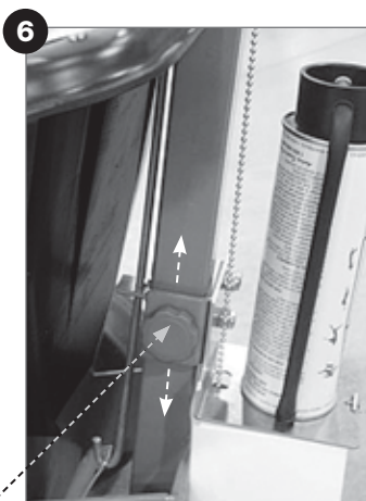
triggering mechanism
