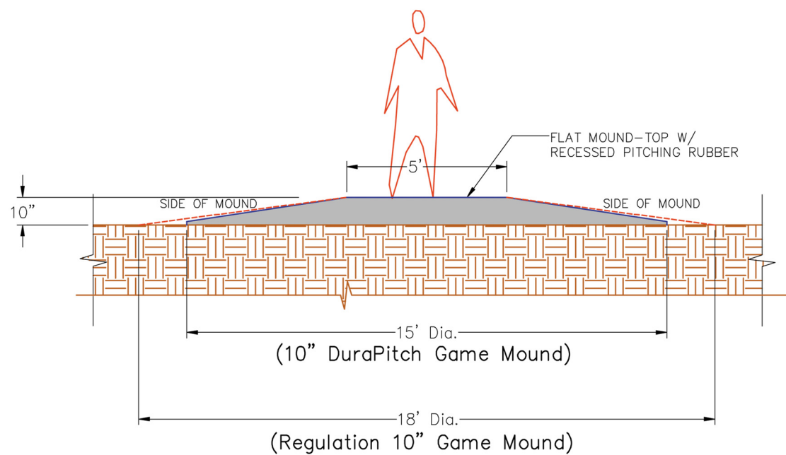
TRANSVERSE SECTION
