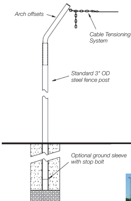
Compatible with chain link enclosures A
